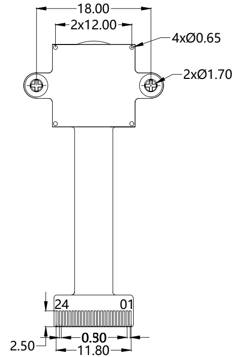
BOTTOM VIEW
